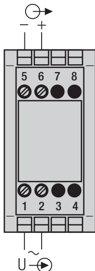
Fig. 2. SINEAX U 543, for AC voltage measurement.
